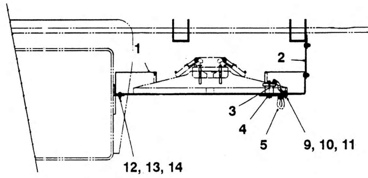
OUTRIGGER FLOAT STOWAGE LEFT HAND
